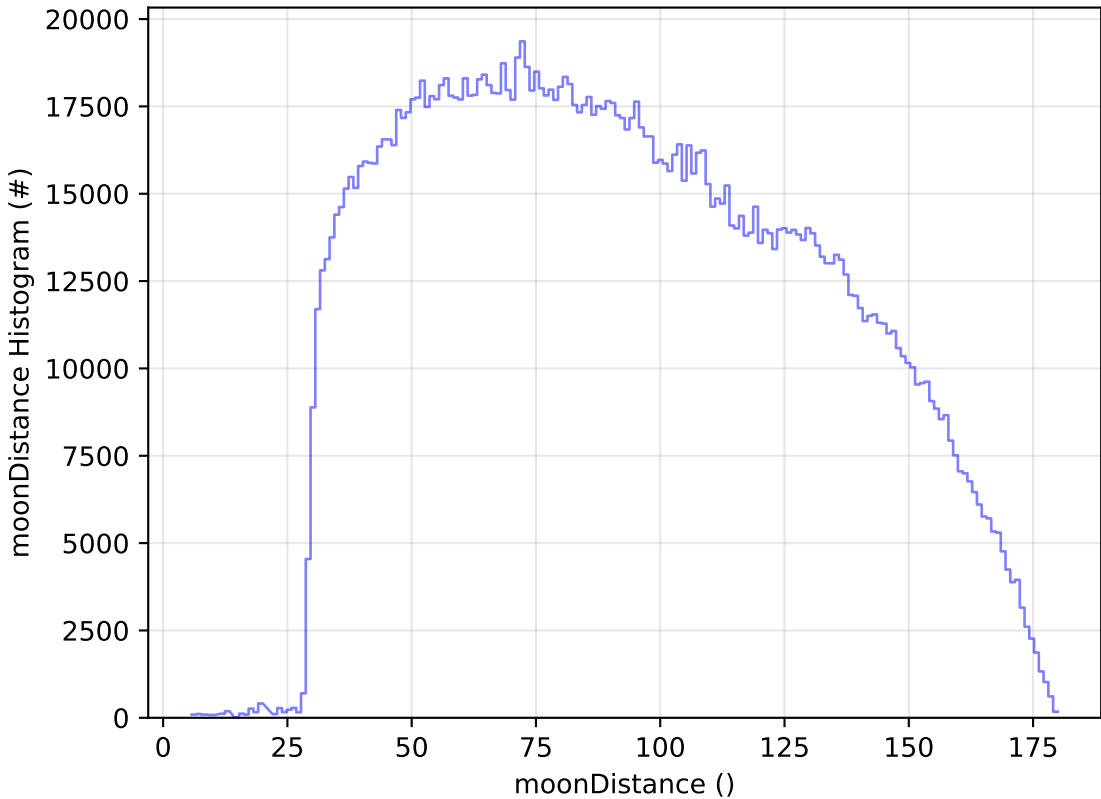
weather_cloudso0v3.4_10yrs WFD all bands: moonDistance Histogram
