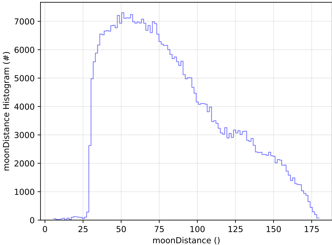
weather_cloudso0v3.4_10yrs All sky z band: moonDistance Histogram
