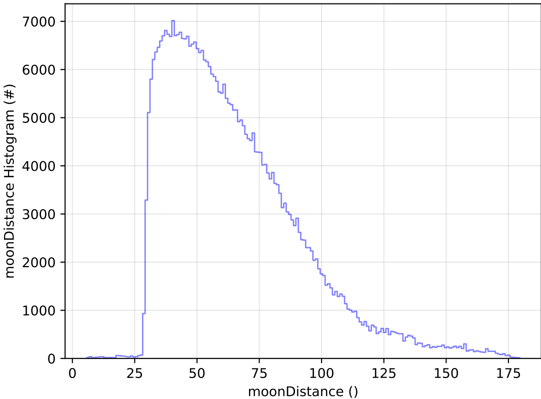
weather_cloudso0v3.4_10yrs All sky y band: moonDistance Histogram
