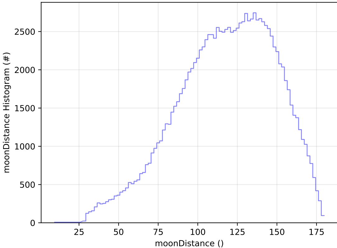
weather_cloudso0v3.4_10yrs All sky u band: moonDistance Histogram
