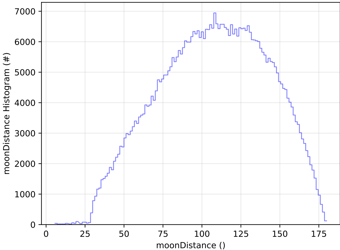
weather_cloudso0v3.4_10yrs All sky r band: moonDistance Histogram
