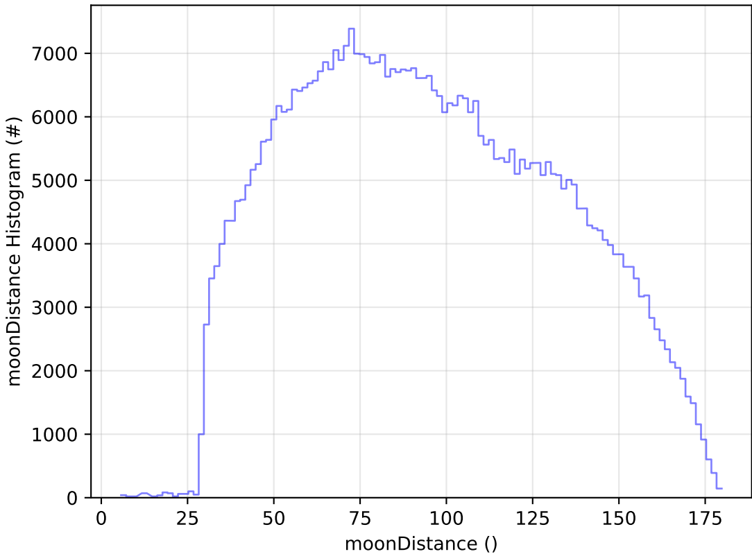
weather_cloudso0v3.4_10yrs All sky i band: moonDistance Histogram
