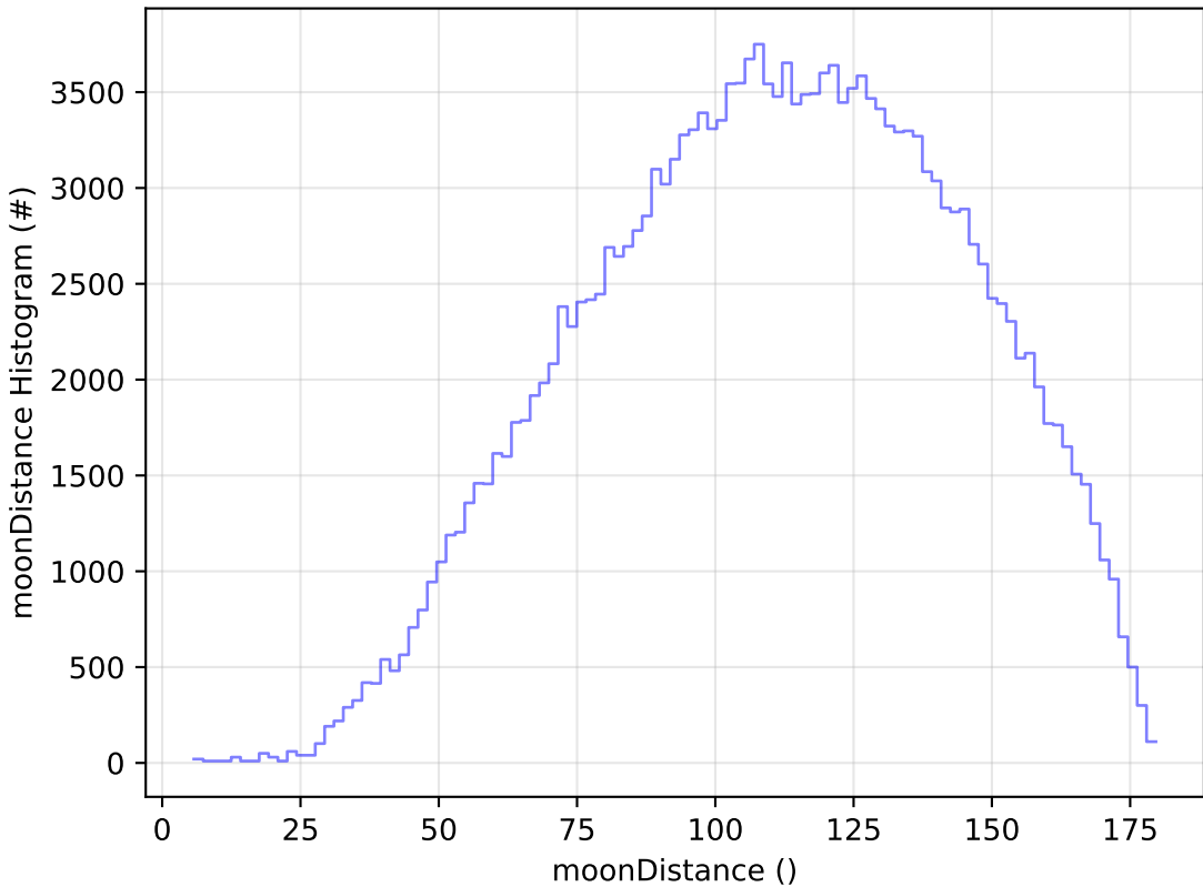
weather_cloudso0v3.4_10yrs All sky g band: moonDistance Histogram
