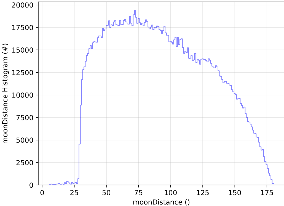
weather_cloudso0v3.4_10yrs All sky all bands: moonDistance Histogram
