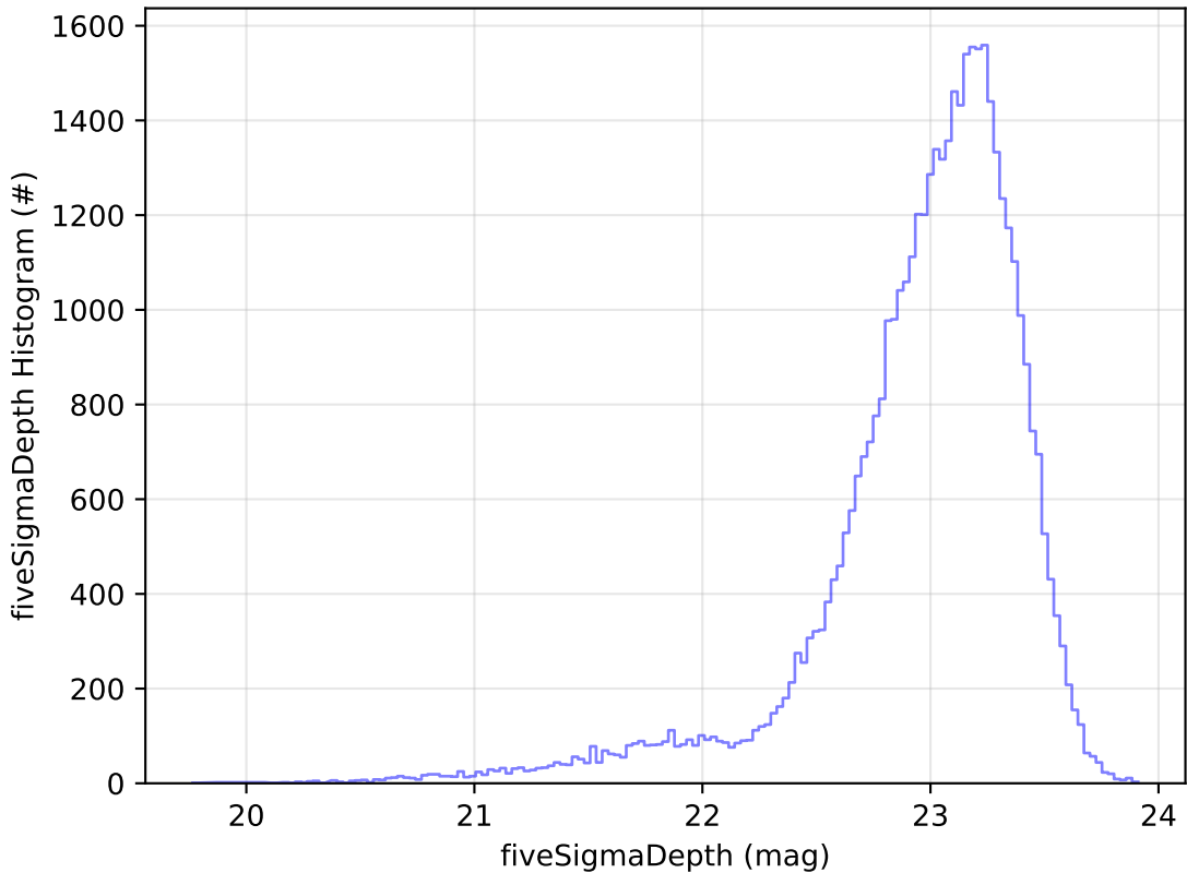
weather_cloudso0v3.4_10yrs Yr 1 z band: fiveSigmaDepth Histogram
