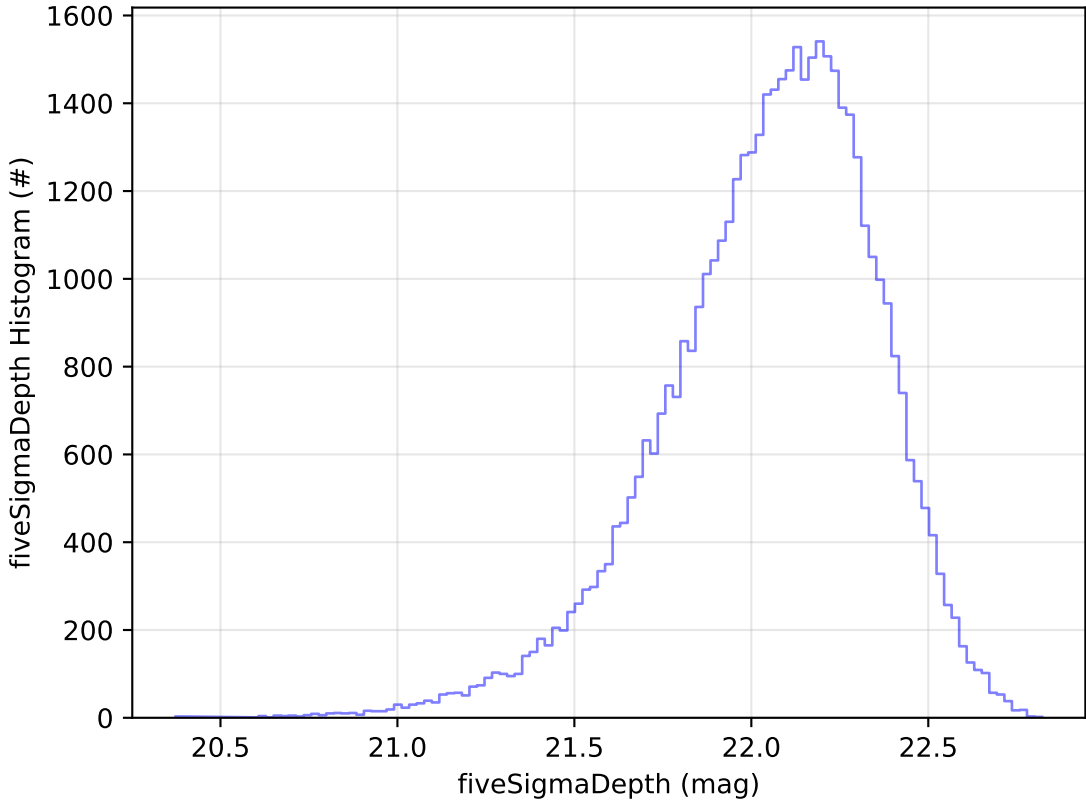
weather_cloudso0v3.4_10yrs Yr 1 y band: fiveSigmaDepth Histogram
