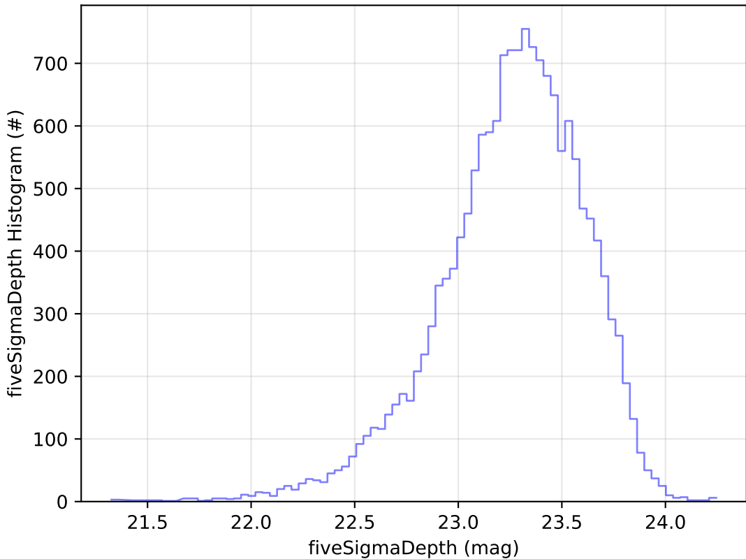
weather_cloudso0v3.4_10yrs Yr 1 u band: fiveSigmaDepth Histogram
