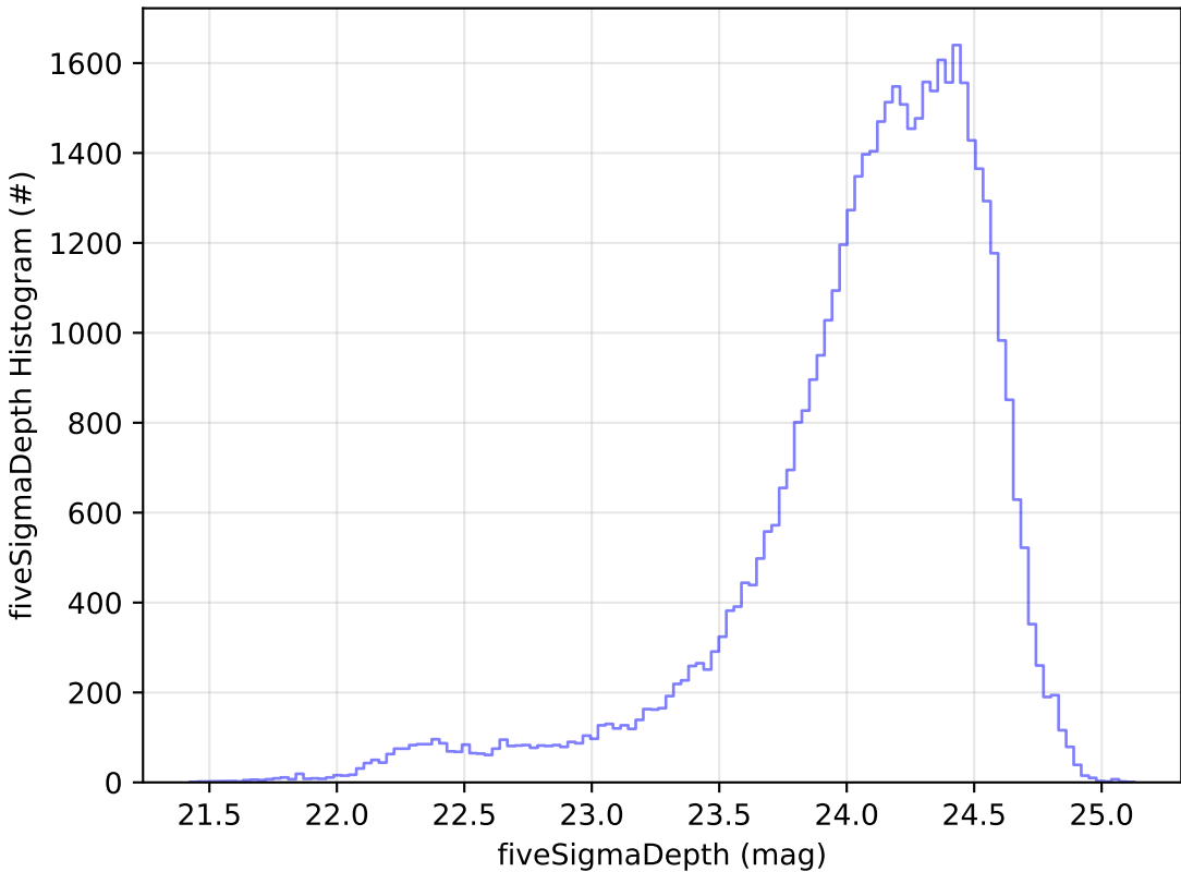
weather_cloudso0v3.4_10yrs Yr 1 r band: fiveSigmaDepth Histogram
