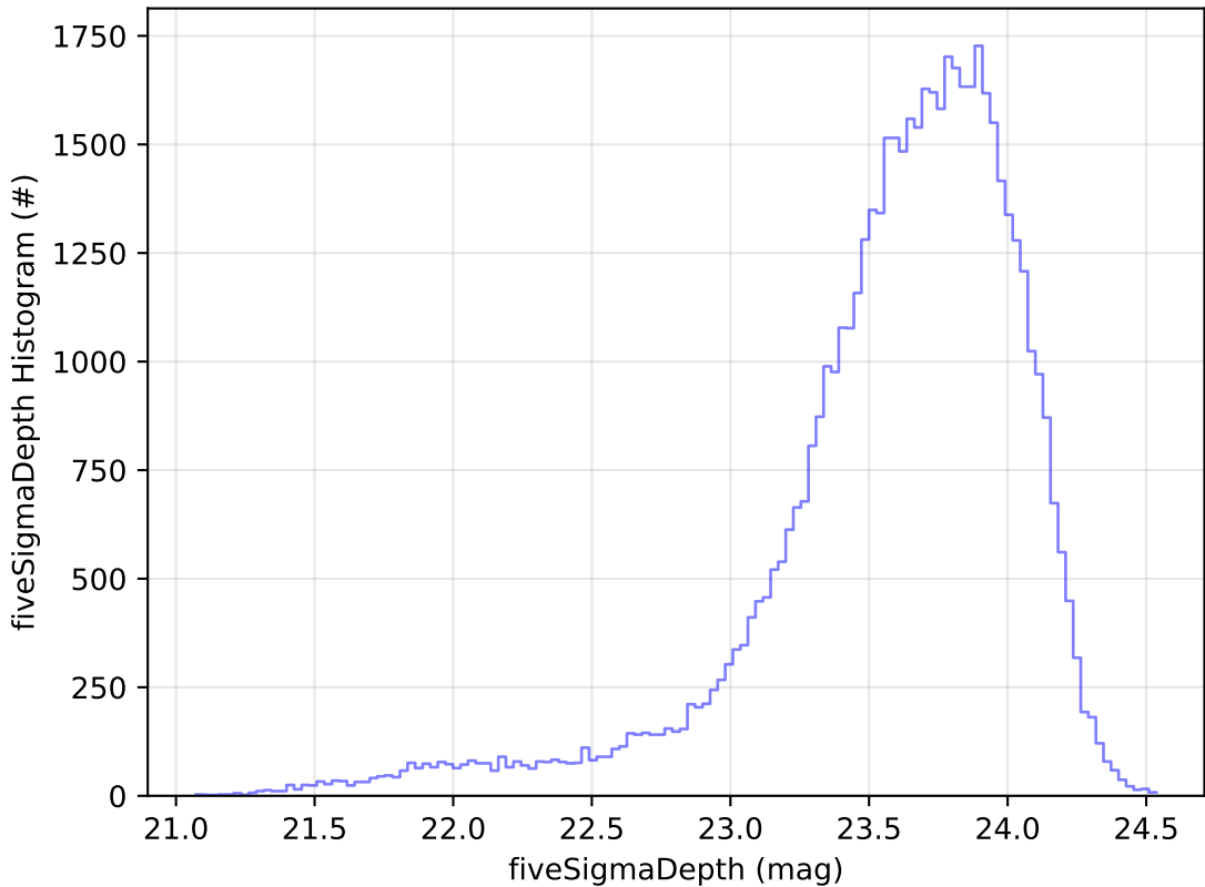
weather_cloudso0v3.4_10yrs Yr 1 i band: fiveSigmaDepth Histogram
