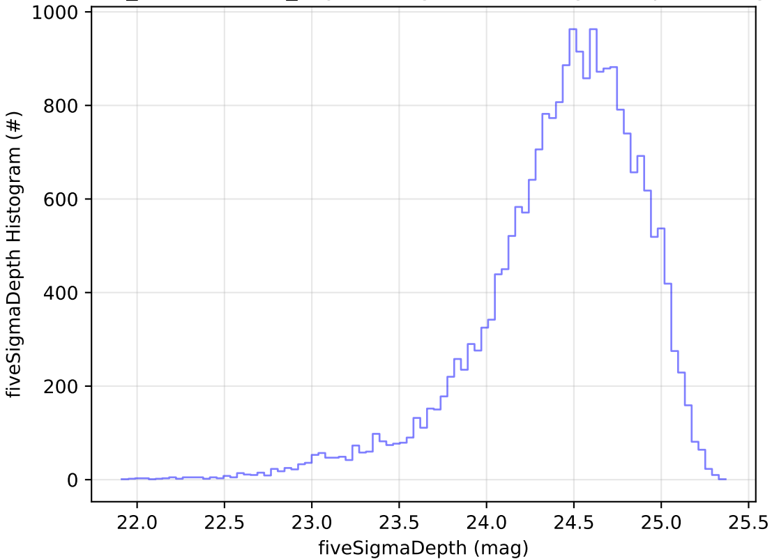
weather_cloudso0v3.4_10yrs Yr 1 g band: fiveSigmaDepth Histogram
