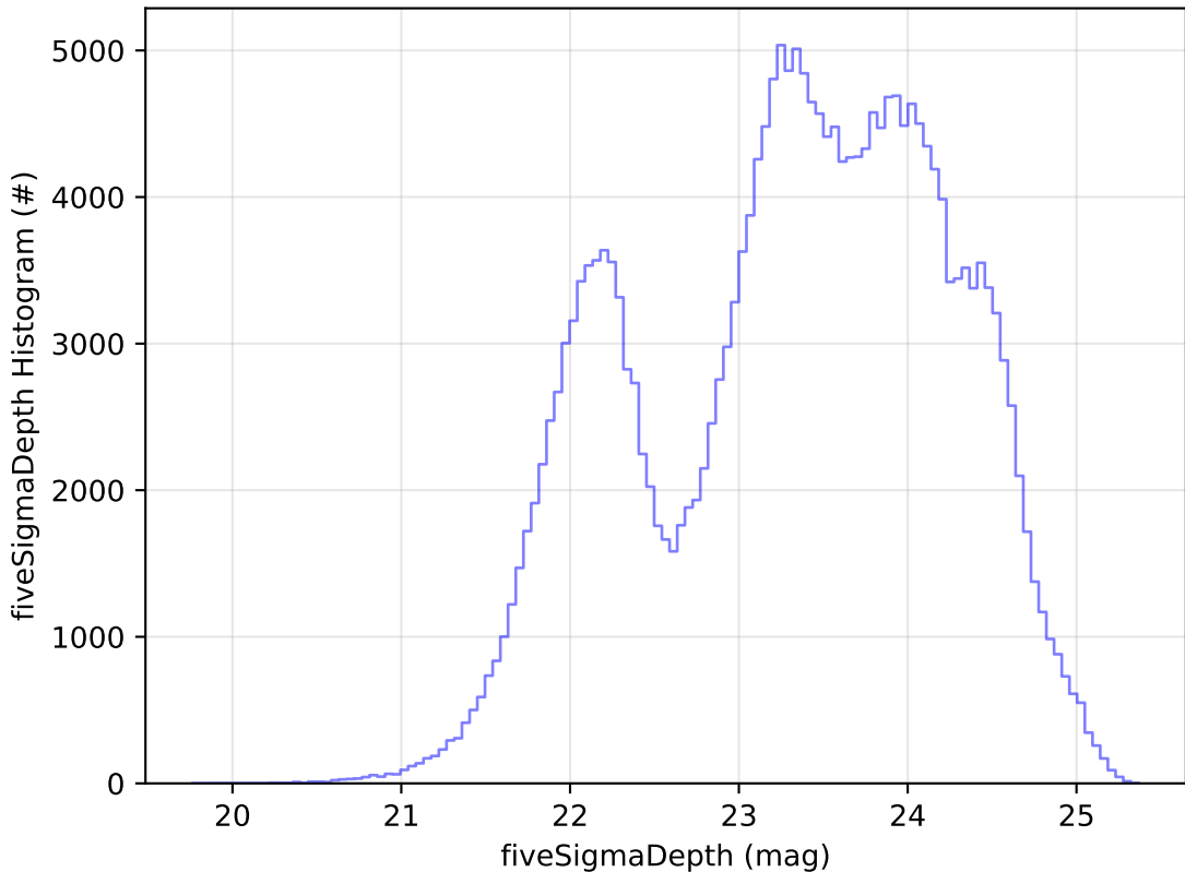
weather_cloudso0v3.4_10yrs Yr 1 all bands: fiveSigmaDepth Histogram
