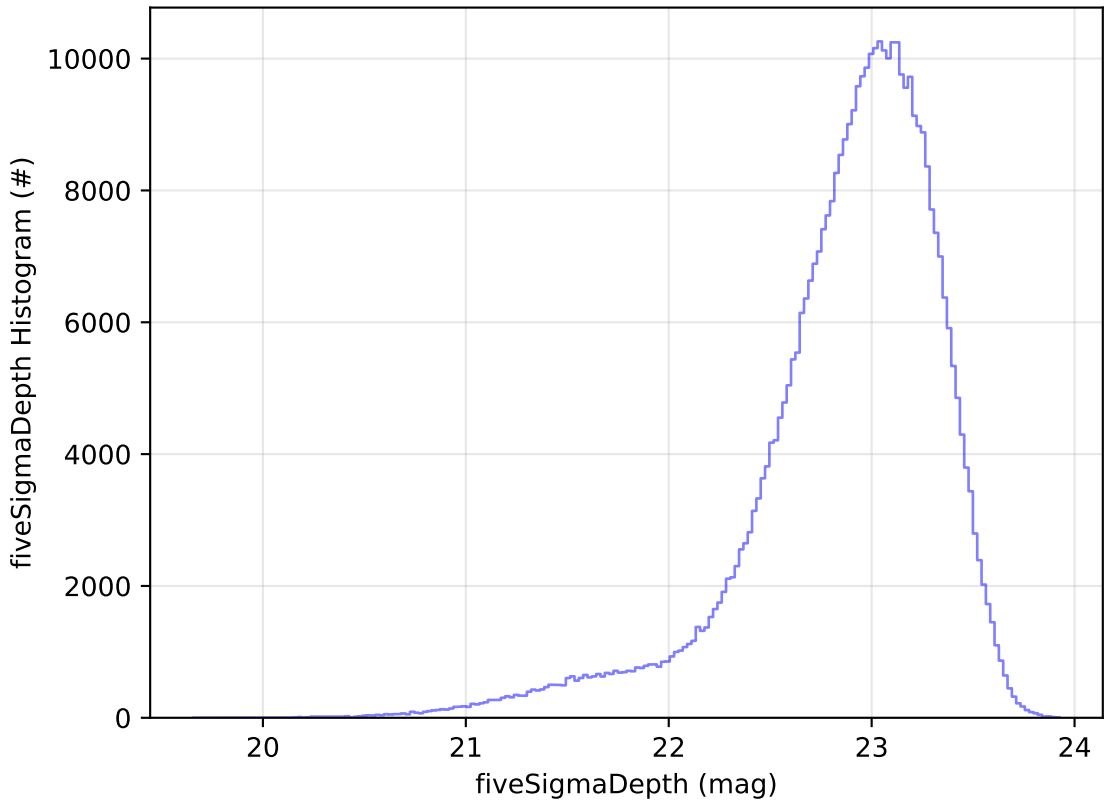
weather_cloudso0v3.4_10yrs WFD z band: fiveSigmaDepth Histogram
