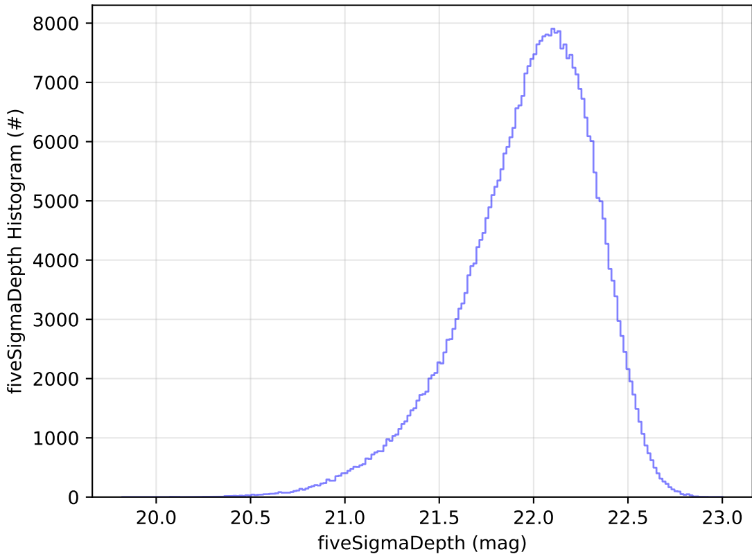
weather_cloudso0v3.4_10yrs WFD y band: fiveSigmaDepth Histogram
