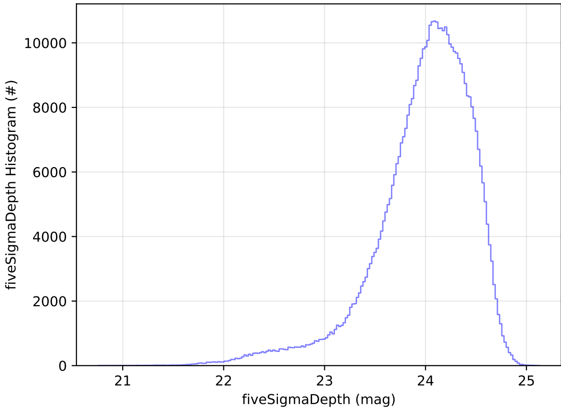
weather_cloudso0v3.4_10yrs WFD r band: fiveSigmaDepth Histogram
