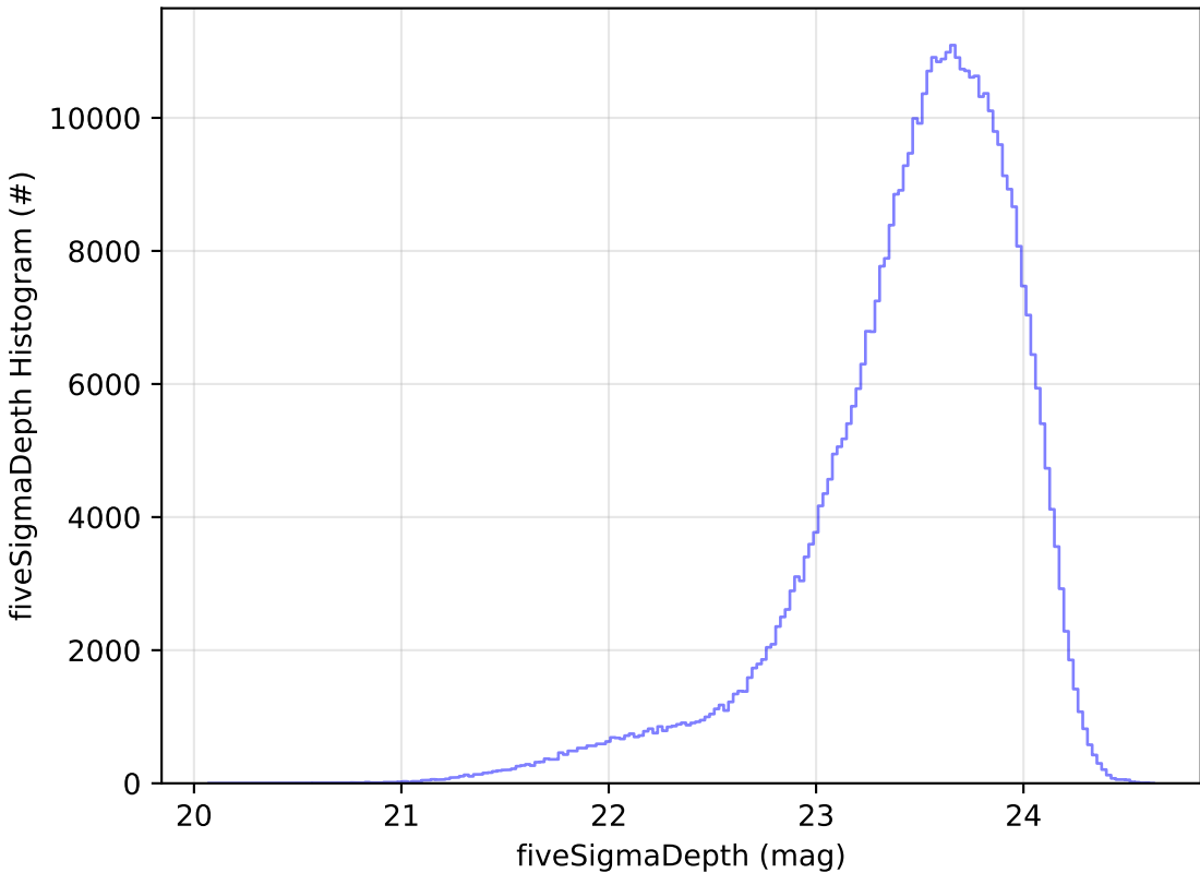
weather_cloudso0v3.4_10yrs WFD i band: fiveSigmaDepth Histogram
