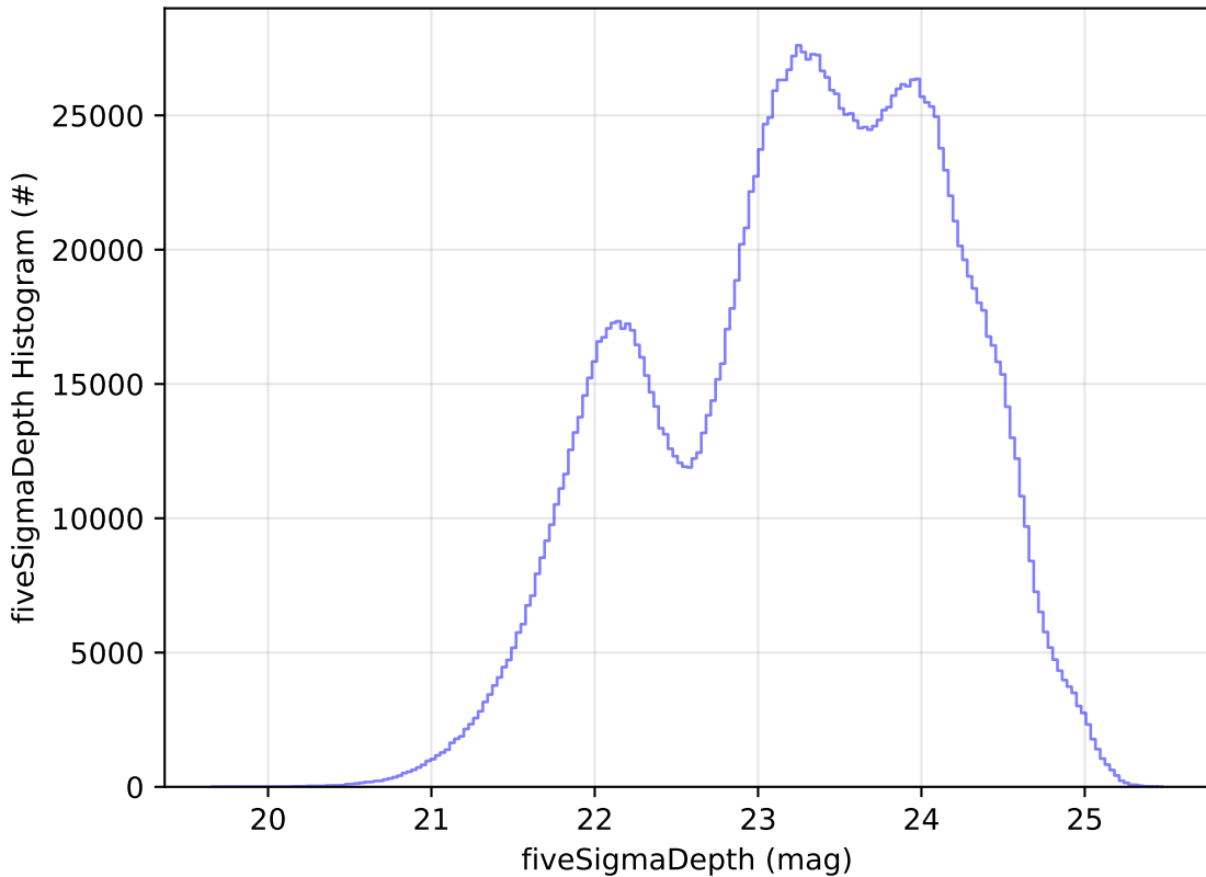
weather_cloudso0v3.4_10yrs WFD all bands: fiveSigmaDepth Histogram
