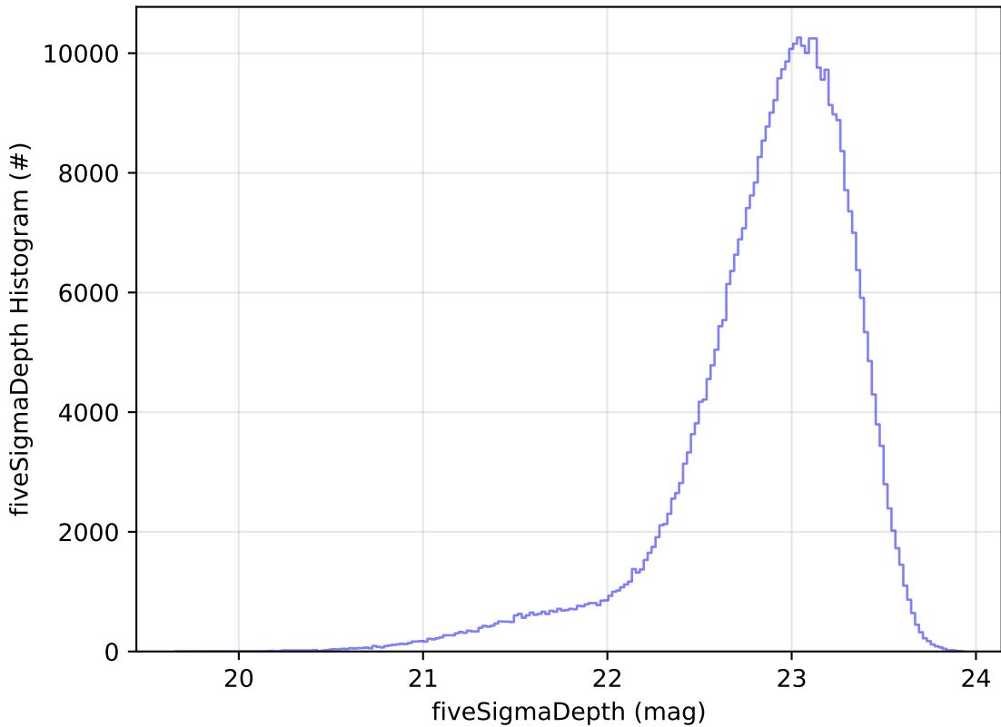
weather_cloudso0v3.4_10yrs All sky z band: fiveSigmaDepth Histogram
