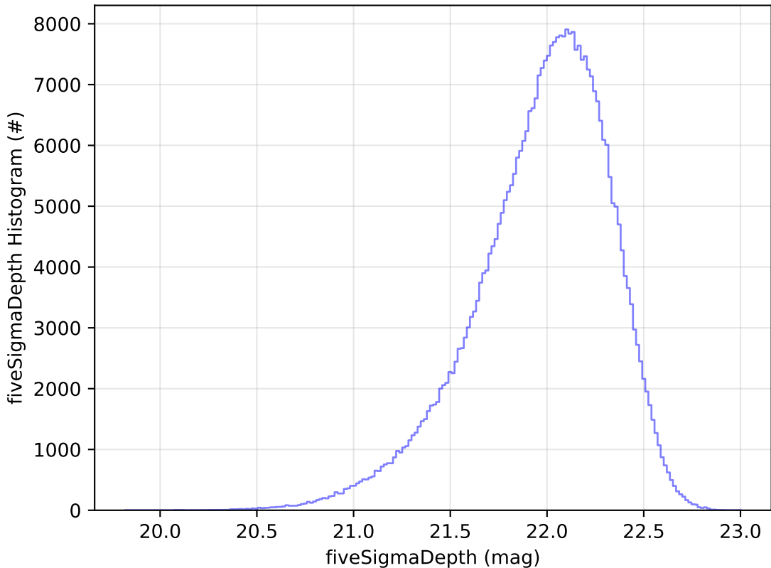
weather_cloudso0v3.4_10yrs All sky y band: fiveSigmaDepth Histogram
