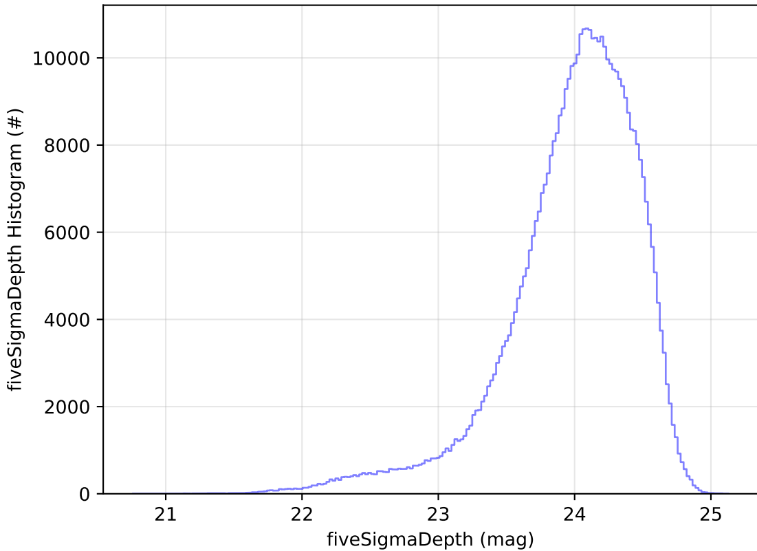
weather_cloudso0v3.4_10yrs All sky r band: fiveSigmaDepth Histogram
