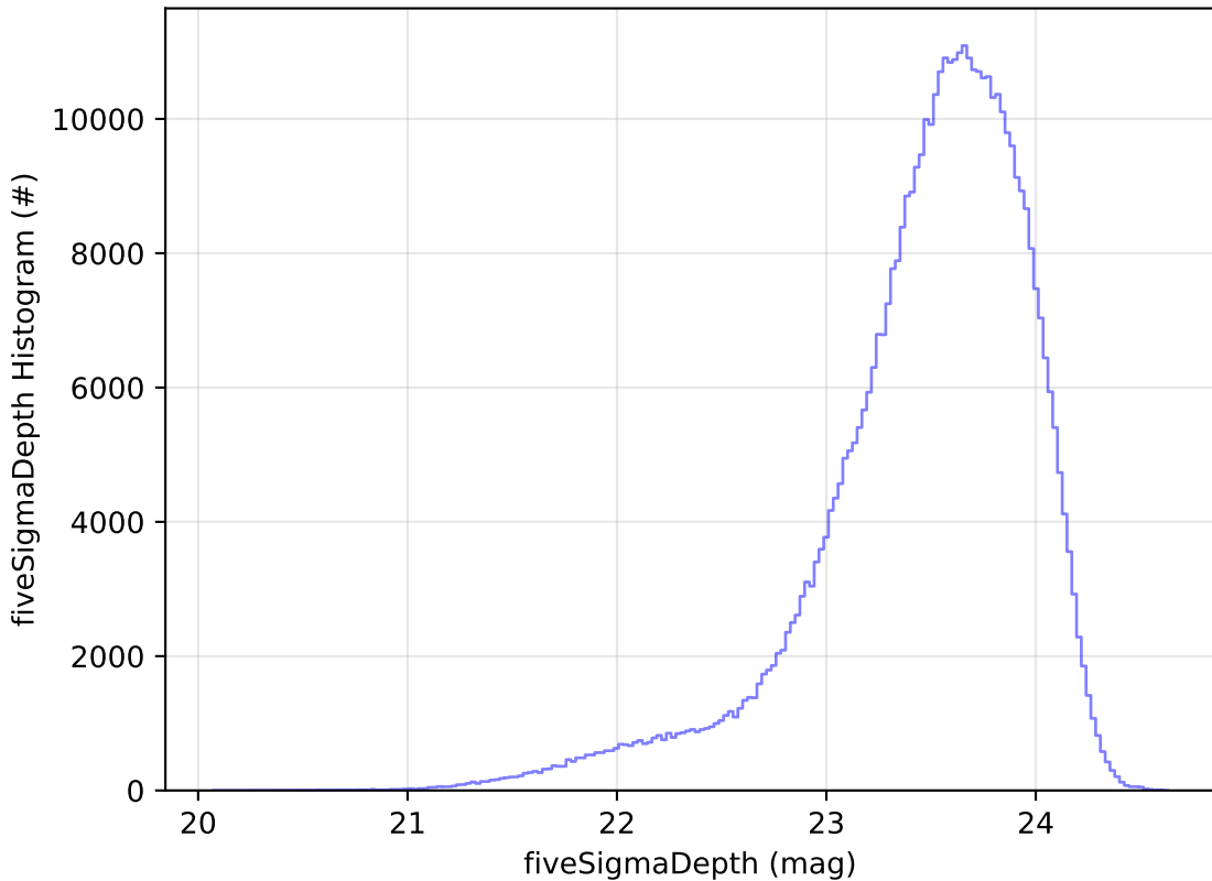
weather_cloudso0v3.4_10yrs All sky i band: fiveSigmaDepth Histogram
