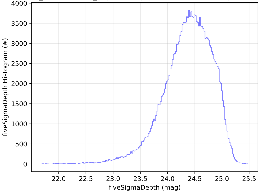
weather_cloudso0v3.4_10yrs All sky g band: fiveSigmaDepth Histogram
