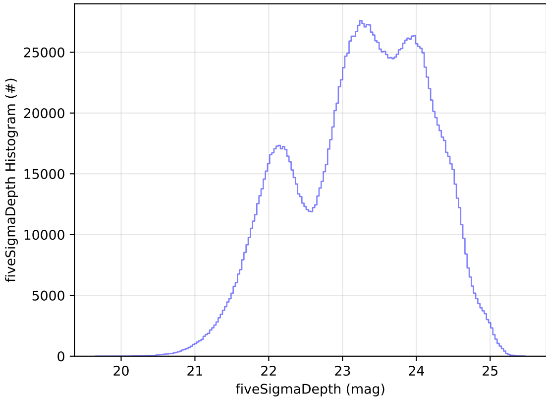
weather_cloudso0v3.4_10yrs All sky all bands: fiveSigmaDepth Histogram
