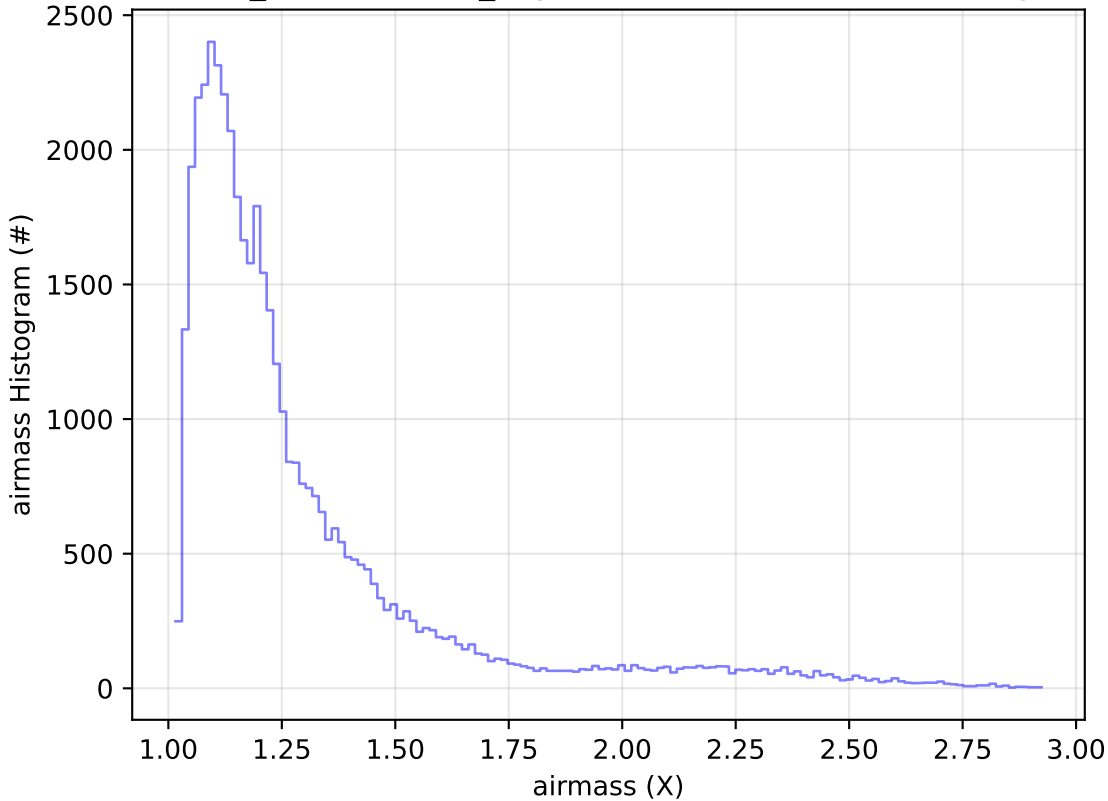
weather_cloudso0v3.4_10yrs Yr 1 z band: airmass Histogram
