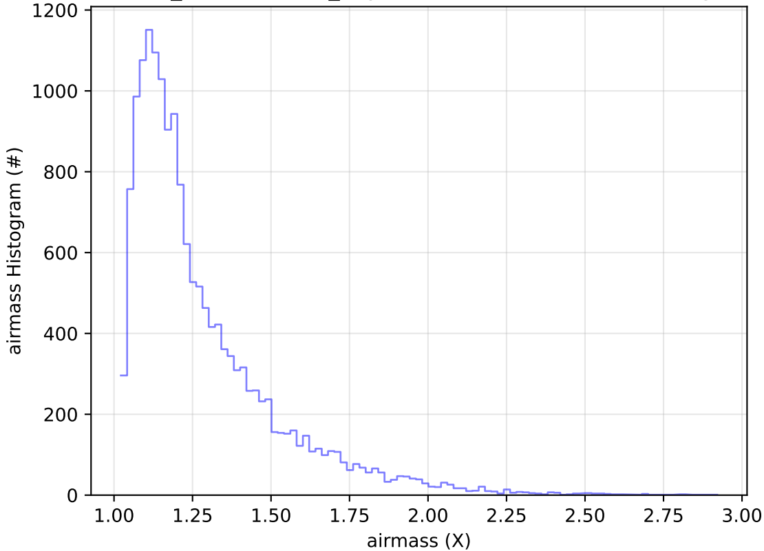
weather_cloudso0v3.4_10yrs Yr 1 u band: airmass Histogram
