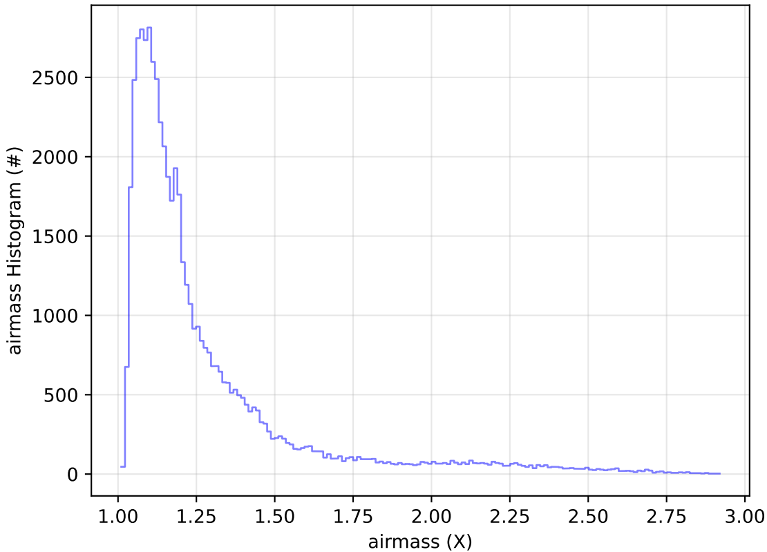
weather_cloudso0v3.4_10yrs Yr 1 i band: airmass Histogram
