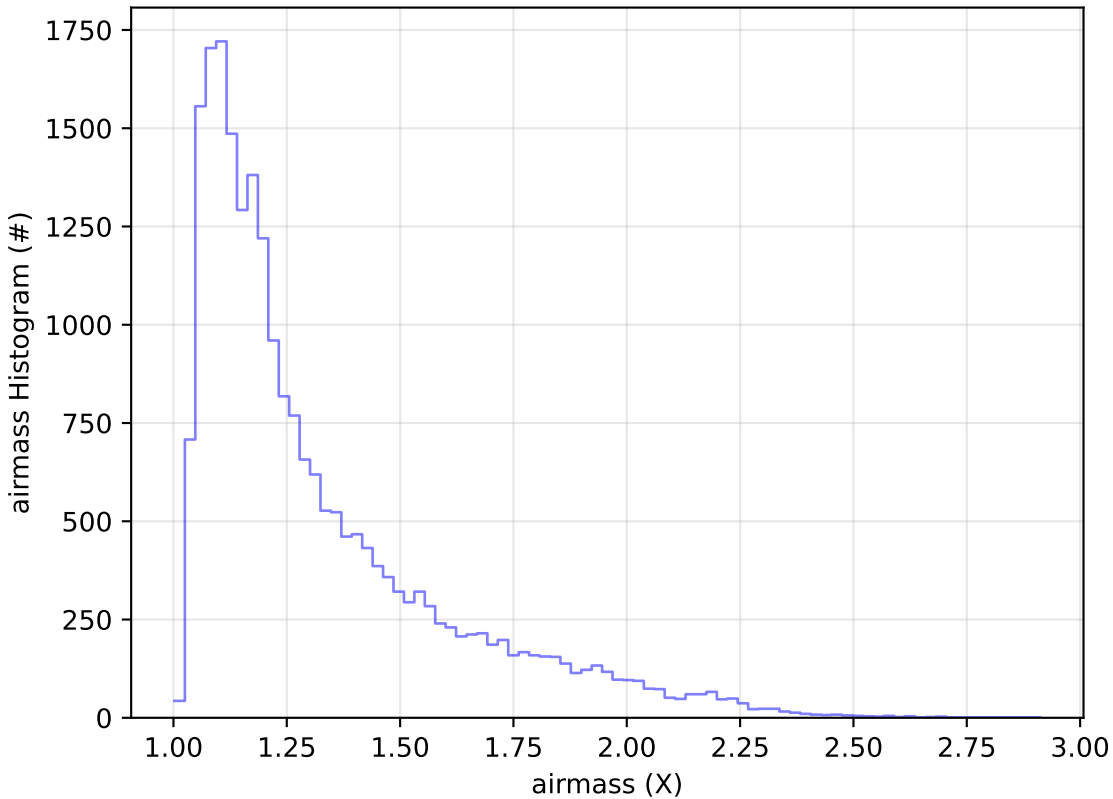
weather_cloudso0v3.4_10yrs Yr 1 g band: airmass Histogram
