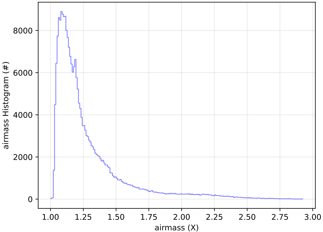
weather_cloudso0v3.4_10yrs Yr 1 all bands: airmass Histogram
