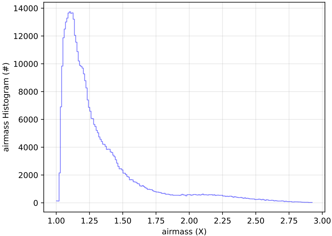
weather_cloudso0v3.4_10yrs WFD z band: airmass Histogram
