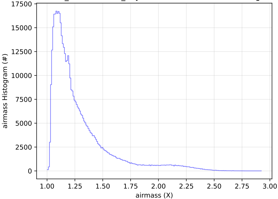
weather_cloudso0v3.4_10yrs WFD r band: airmass Histogram
