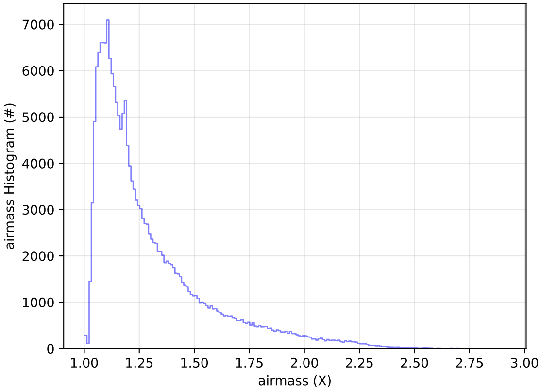
weather_cloudso0v3.4_10yrs WFD g band: airmass Histogram
