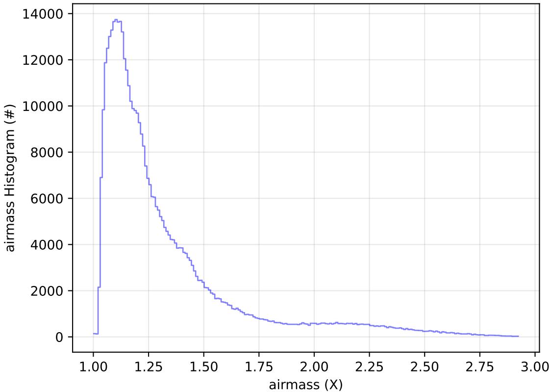
weather_cloudso0v3.4_10yrs All sky z band: airmass Histogram
