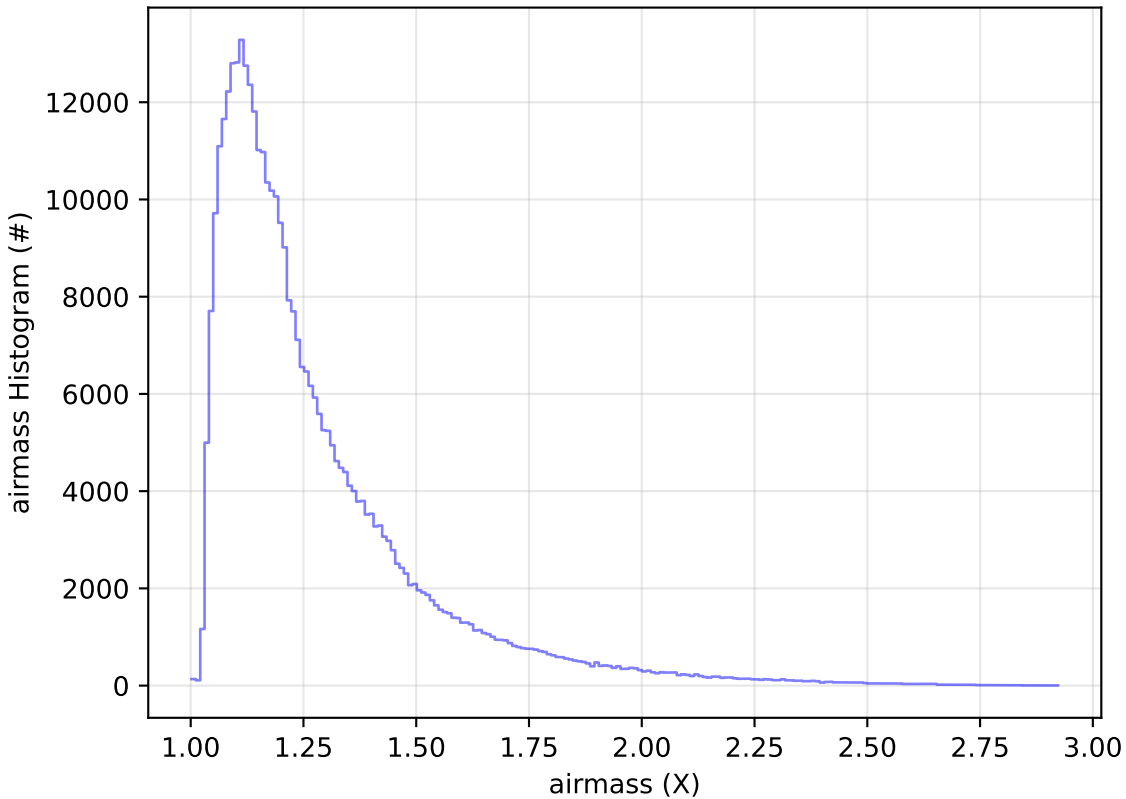
weather_cloudso0v3.4_10yrs All sky y band: airmass Histogram
