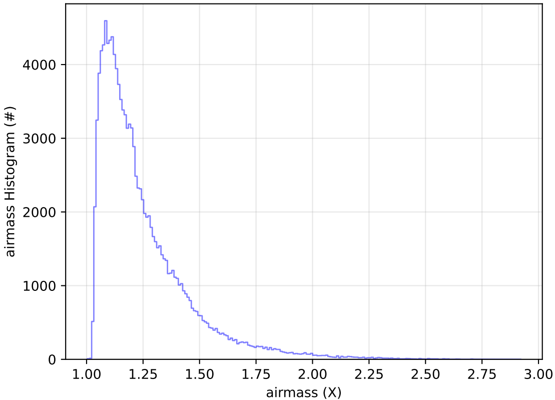
weather_cloudso0v3.4_10yrs All sky u band: airmass Histogram
