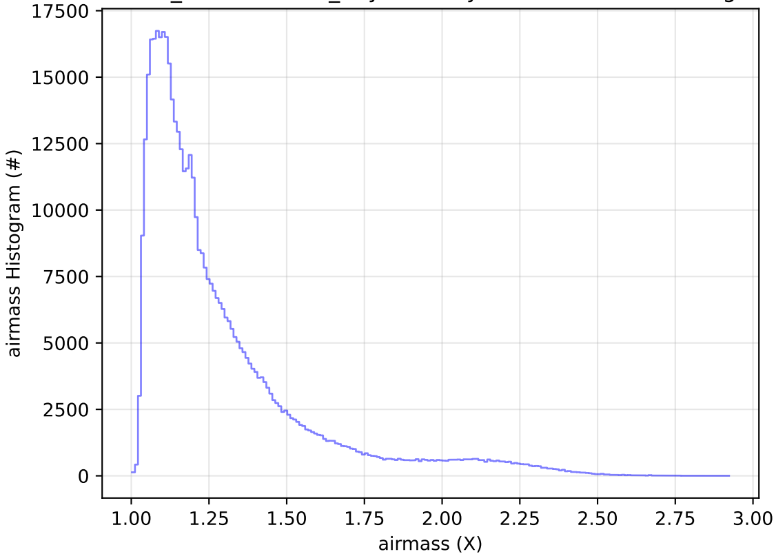
weather_cloudso0v3.4_10yrs All sky r band: airmass Histogram
