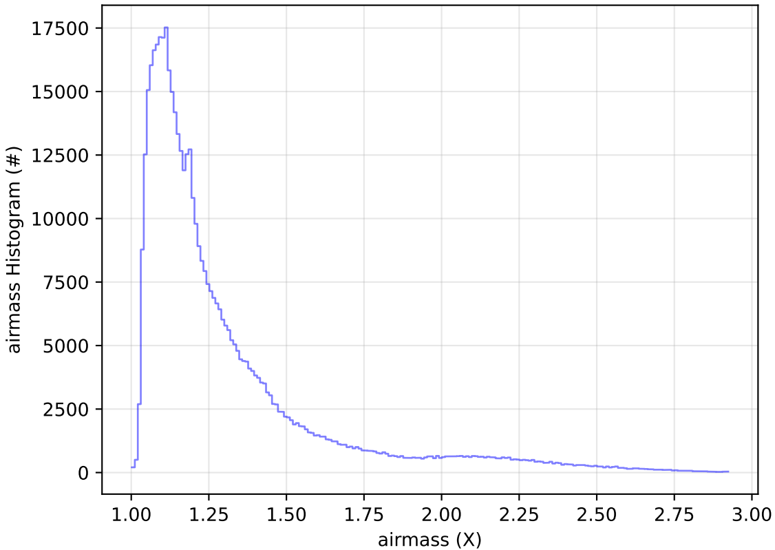
weather_cloudso0v3.4_10yrs All sky i band: airmass Histogram
