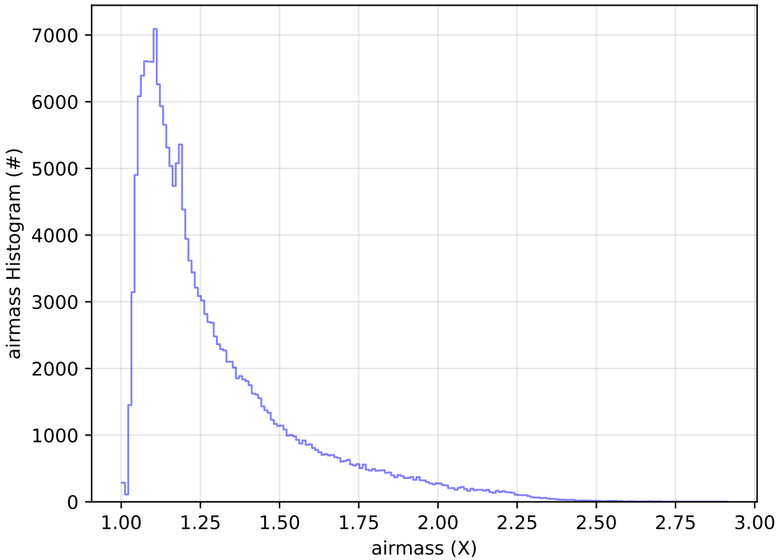
weather_cloudso0v3.4_10yrs All sky g band: airmass Histogram
