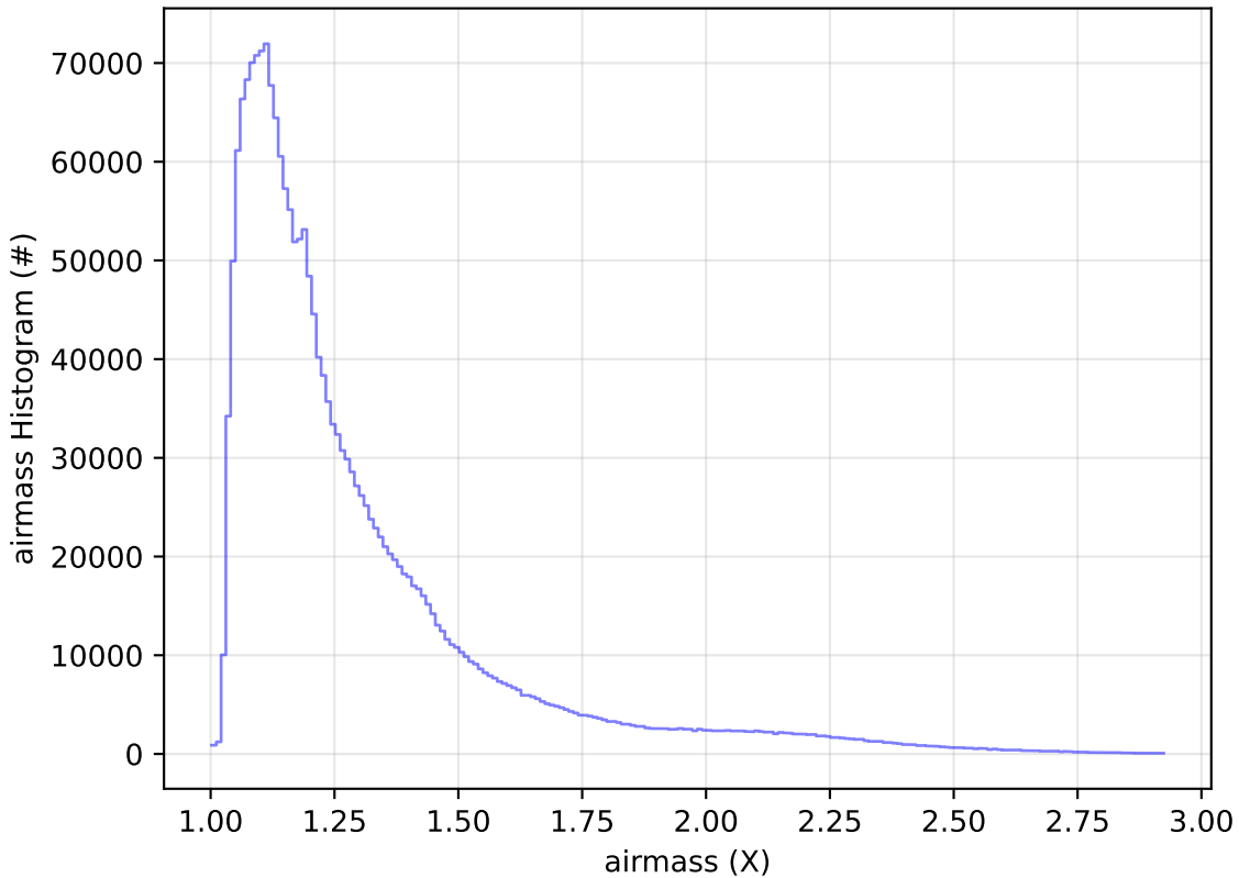
weather_cloudso0v3.4_10yrs All sky all bands: airmass Histogram
