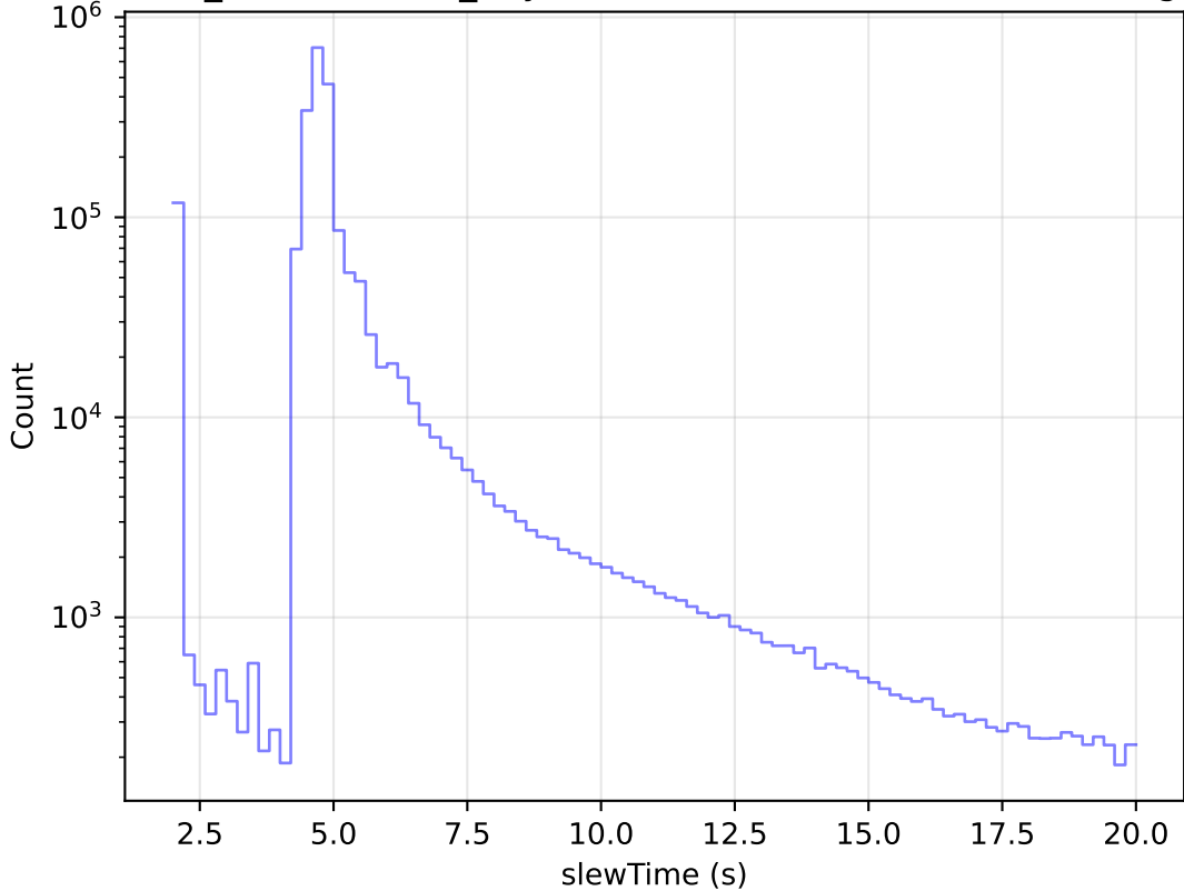
weather_cloudso0v3.4_10yrs All visits: Zoom Slew Time Histogram
