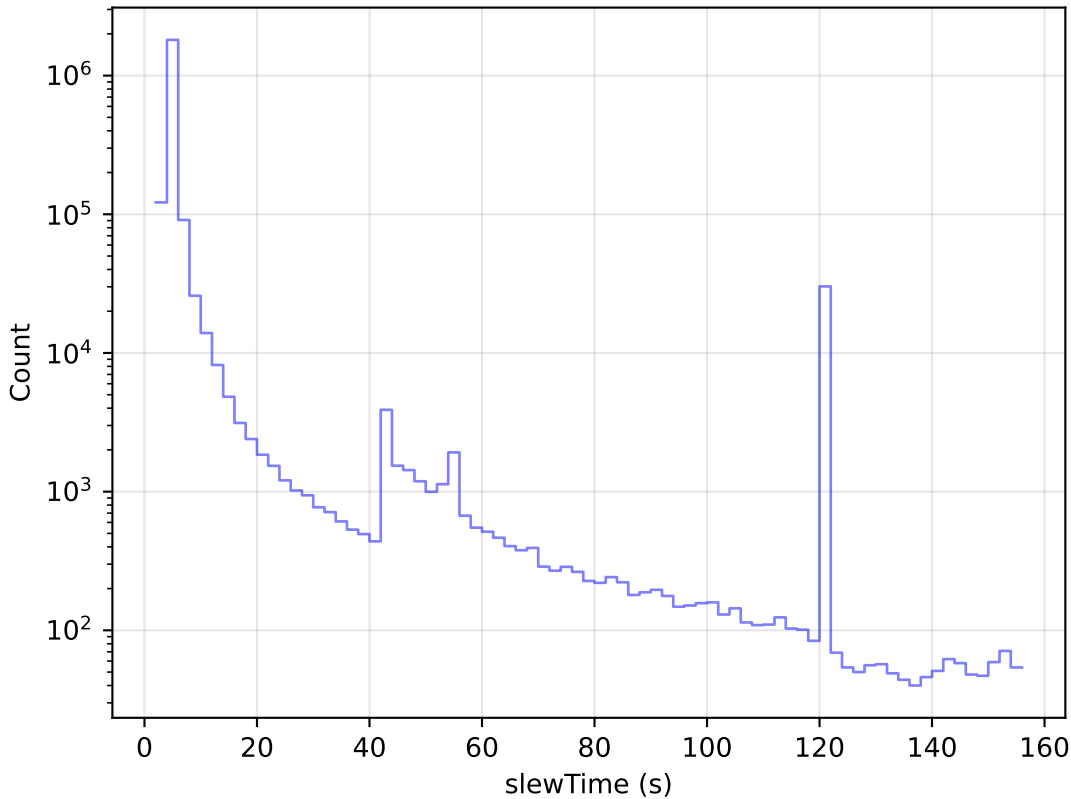
weather_cloudso0v3.4_10yrs All visits: Slew Time Histogram
