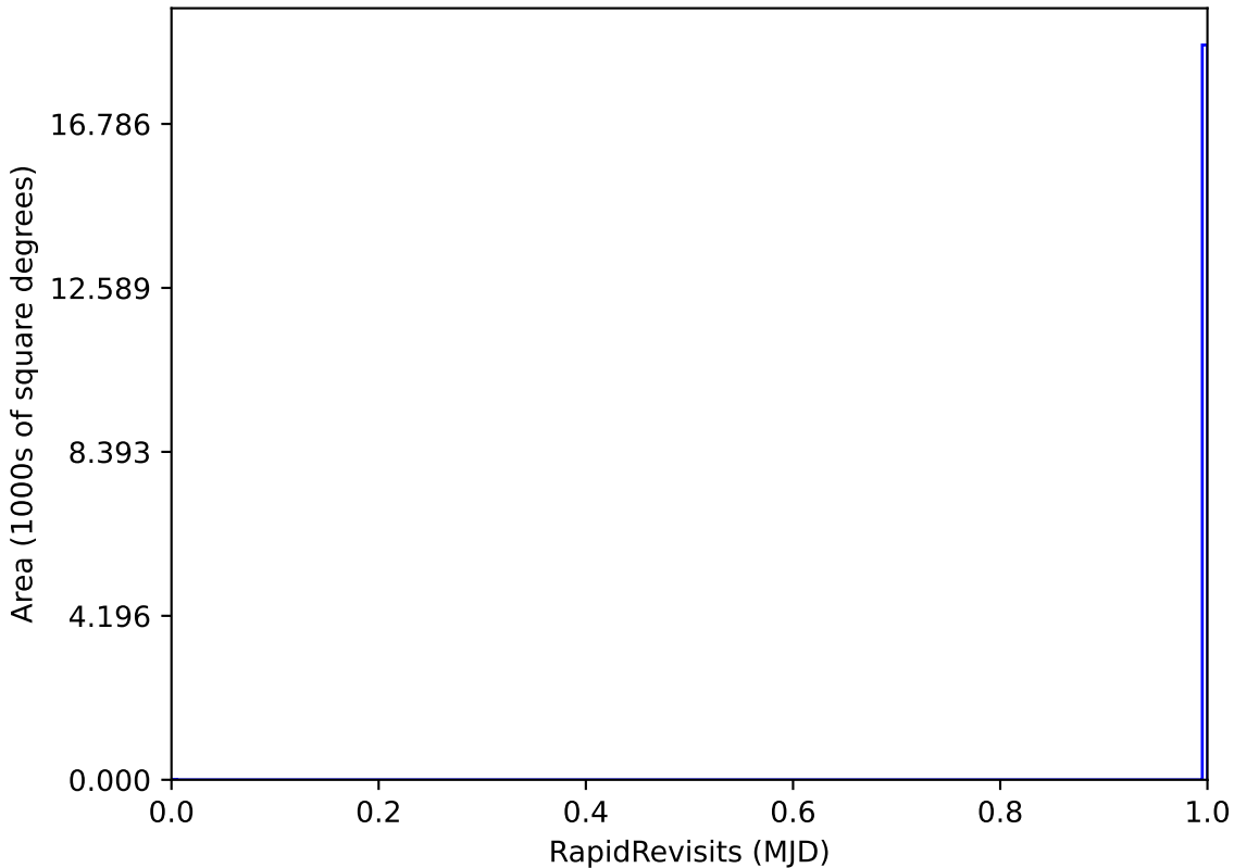
weather_cloudso0v3.4_10yrs WFD: RapidRevisits
