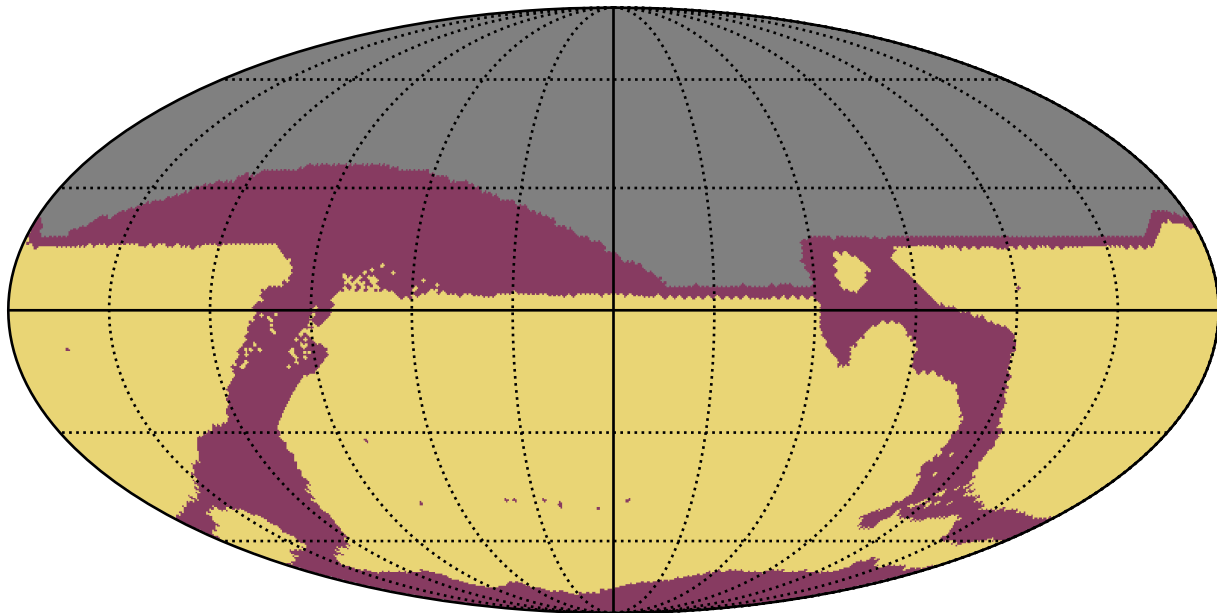
weather_cloudso0v3.4_10yrs All sky: RapidRevisits
