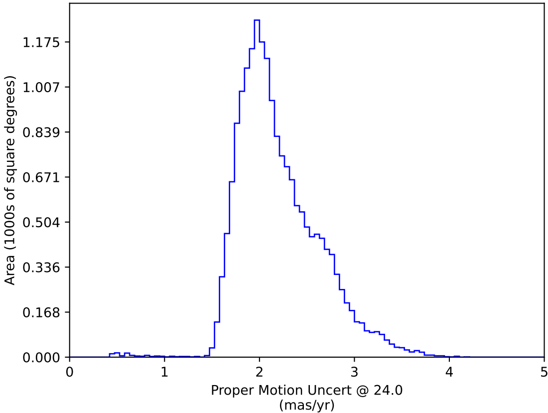
weather_cloudso0v3.4_10yrs WFD: Proper Motion Uncert @ 24.0
