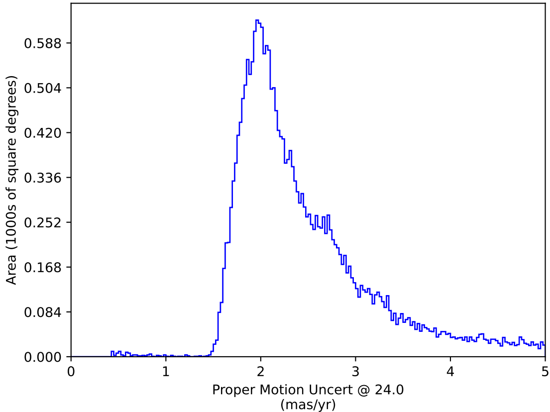
weather_cloudso0v3.4_10yrs All sky: Proper Motion Uncert @ 24.0
