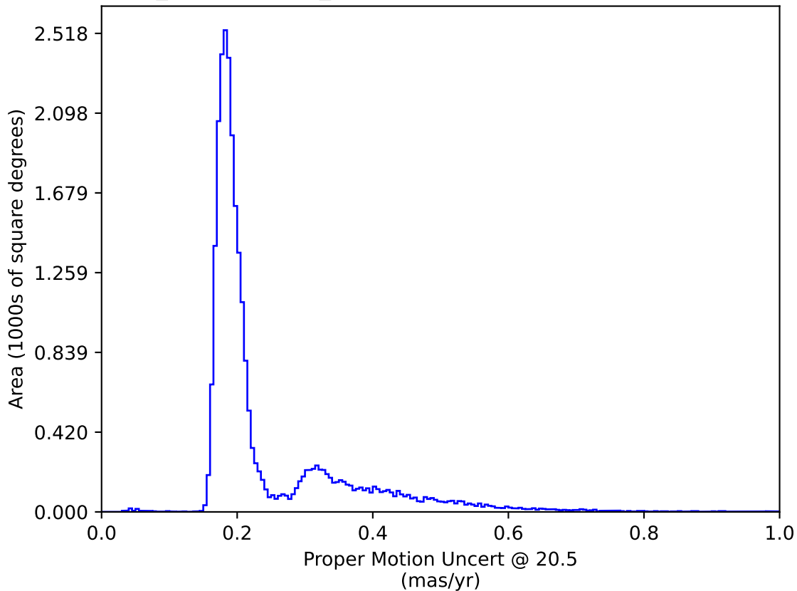
weather_cloudso0v3.4_10yrs All sky: Proper Motion Uncert @ 20.5
