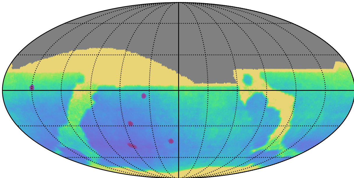
weather_cloudso0v3.4_10yrs All sky: Parallax Uncert @ 24.0
