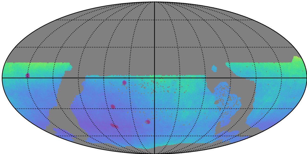
weather_cloudso0v3.4_10yrs WFD: Parallax Uncert @ 22.4
